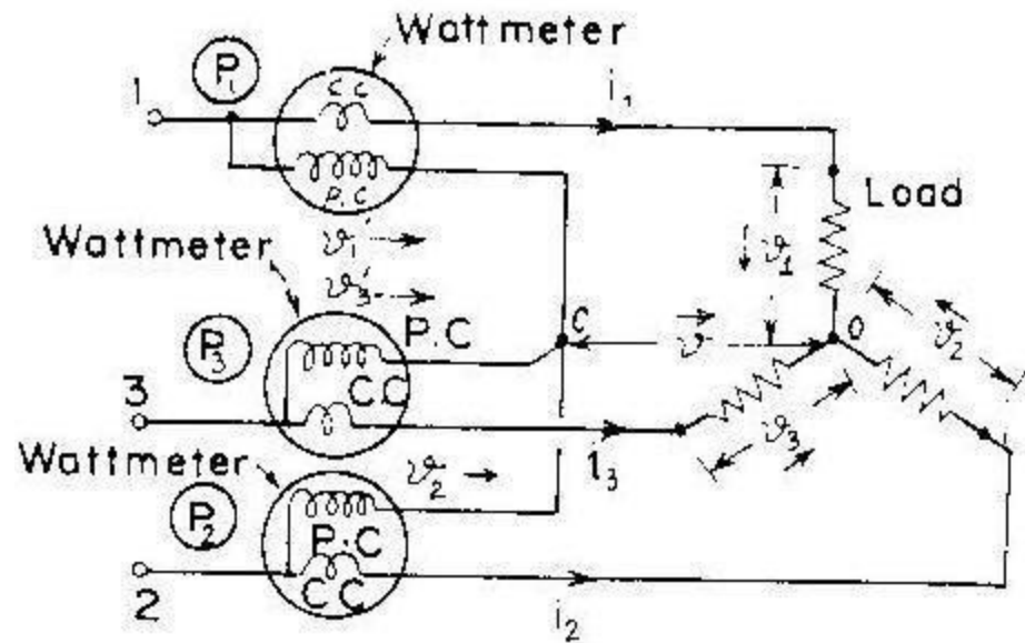
Fig. 11.23. Power measurement in a 3 phase 3 wire system.
