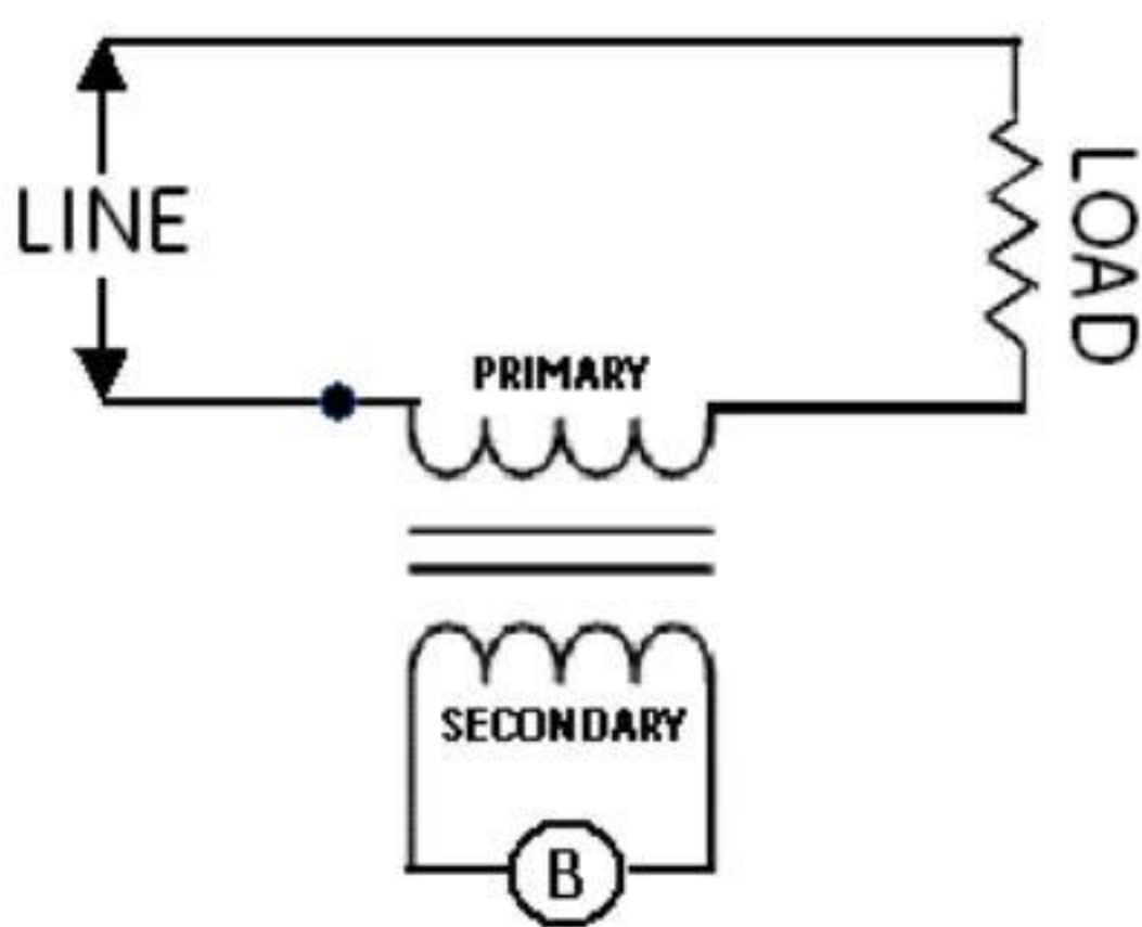
Single-Ratio CT
