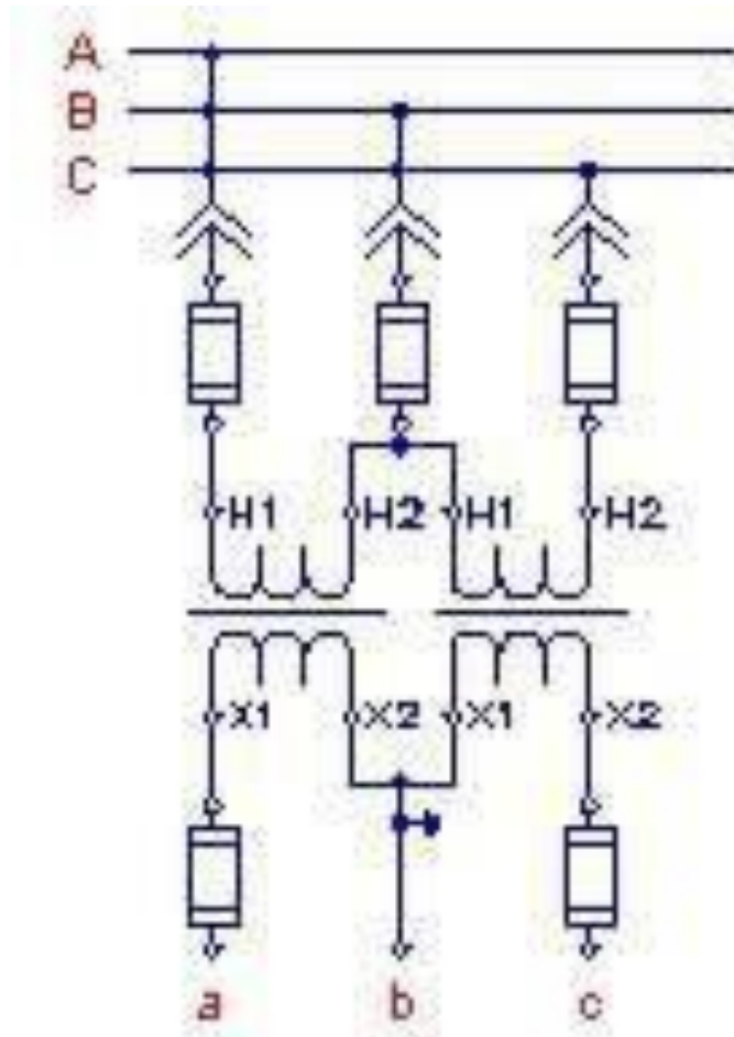
Open Delta Connection (2) Double Bushing VTs
