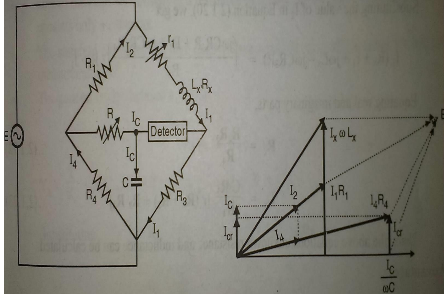
Fig. 2.1.4 : Anderson's bridge
