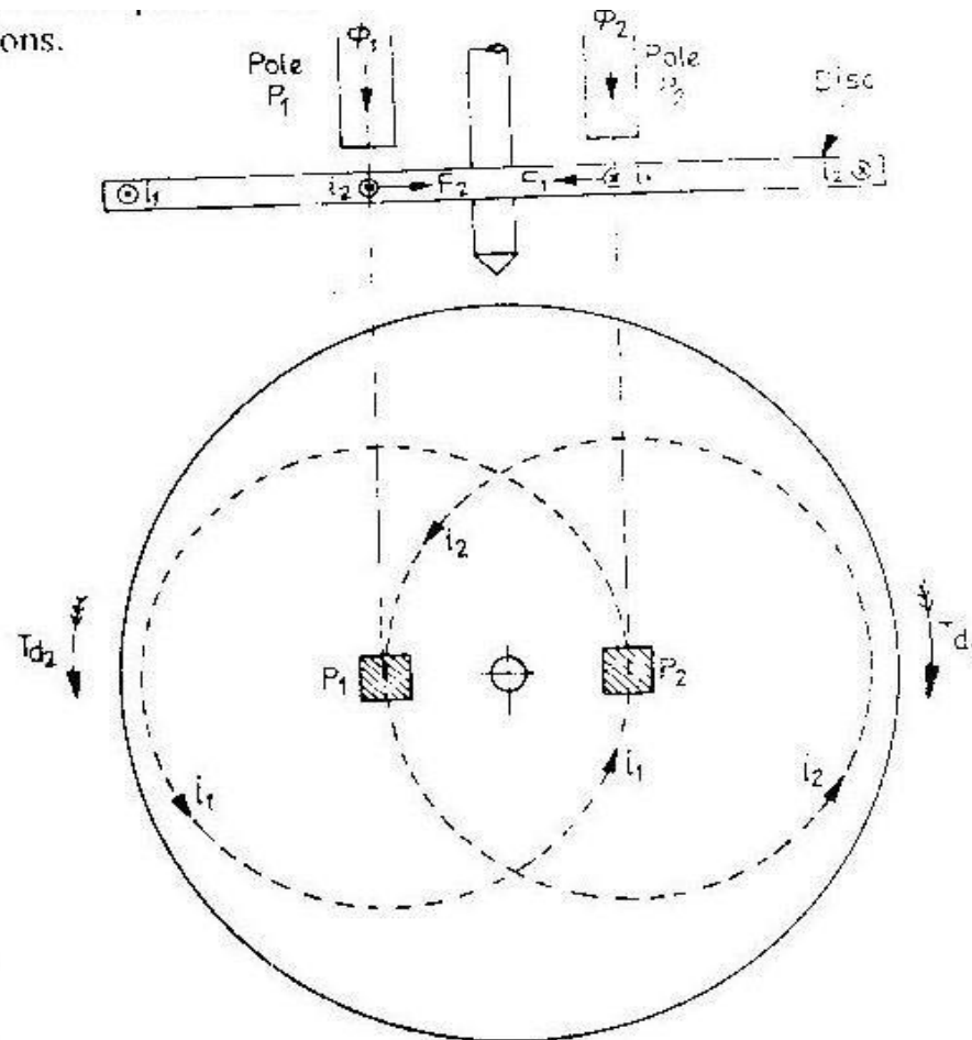
Fig. 12.1. Principle of working of an induction type instrument.
