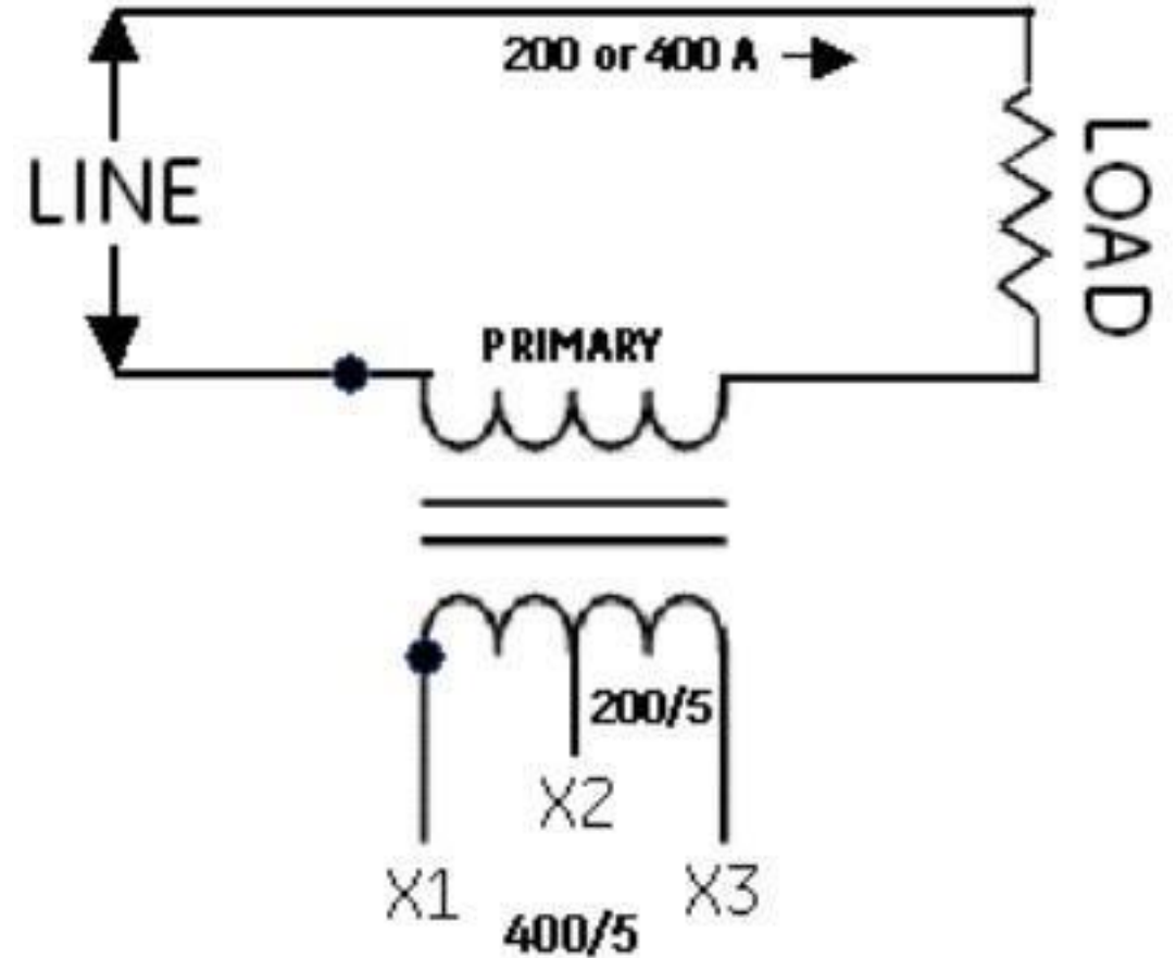
Multi-Ratio CT
