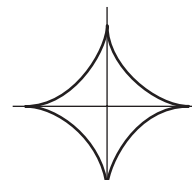
(f) Astroid
