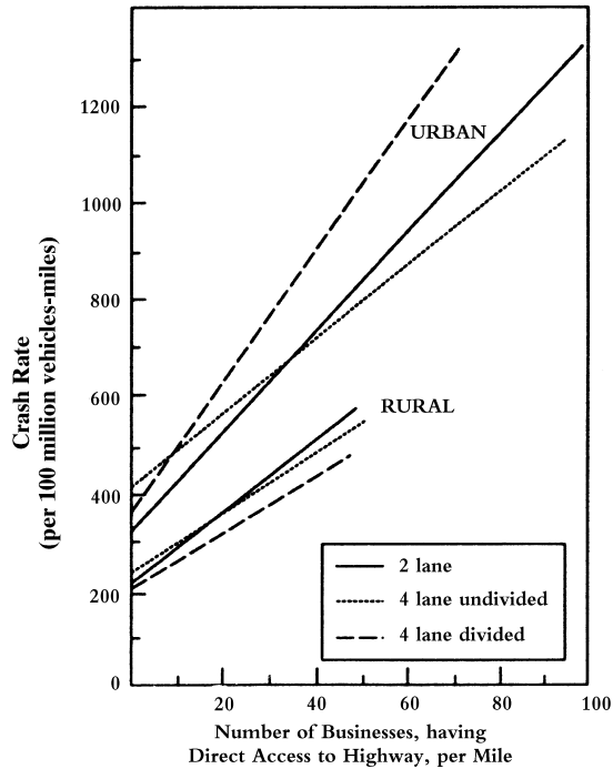
Figure 5.5 Effect of Business Access on Crash Rates on Noninterstate Highways
