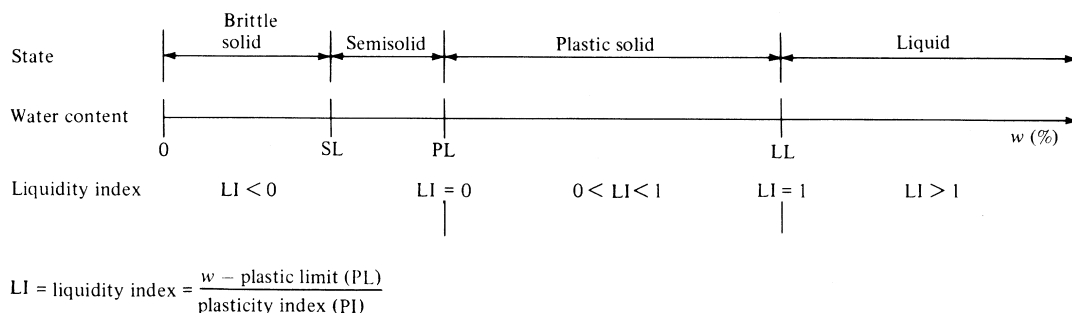
Figure 17.4 Consistency Limits
