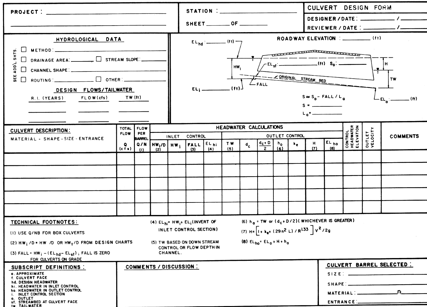
Figure 16.25 Work Sheet for Culvert Design
