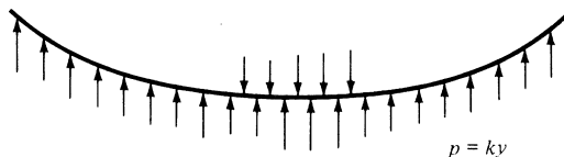
Figure 20.5 Deformation of a Beam on Elastic Foundation
