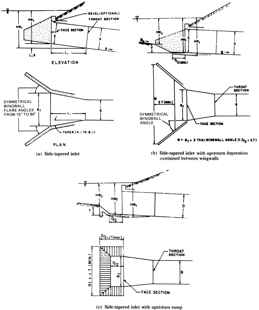
Figure 16.27 Side-Tapered Inlets
