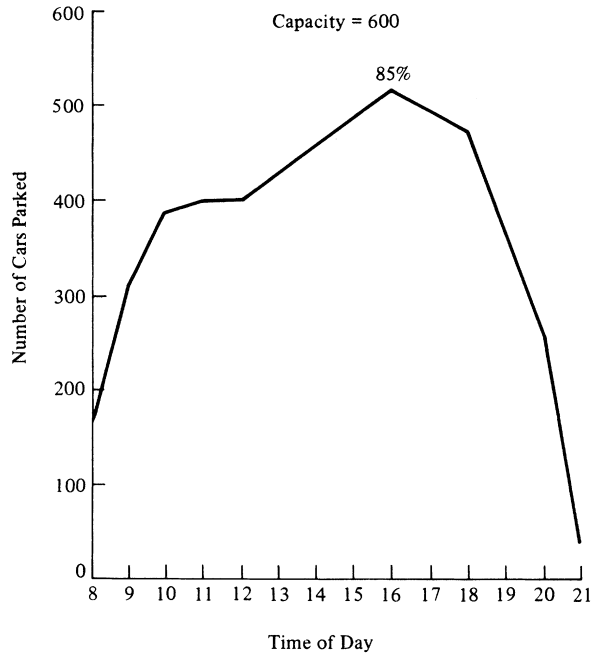
Figure 4.17 Parking Accumulation at a Parking Lot
