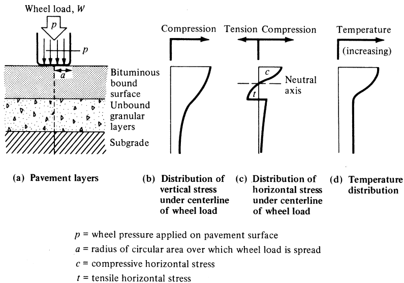
Figure 19.2 Stress Distribution within a Flexible Pavement
