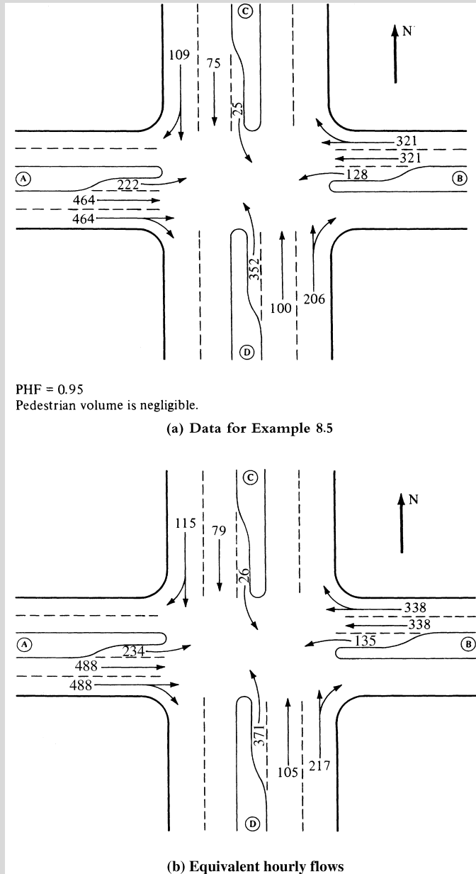
Figure 8.12 Signal Timing Using the Webster Method
