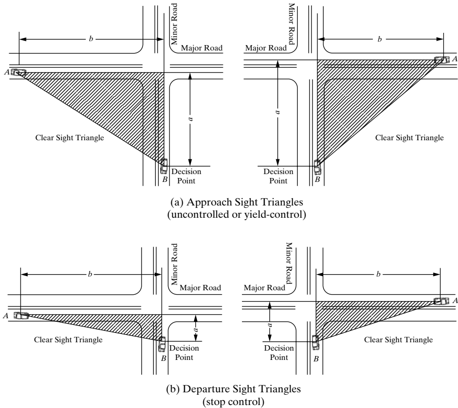
Figure 7.19 Sight Triangles at Intersections
