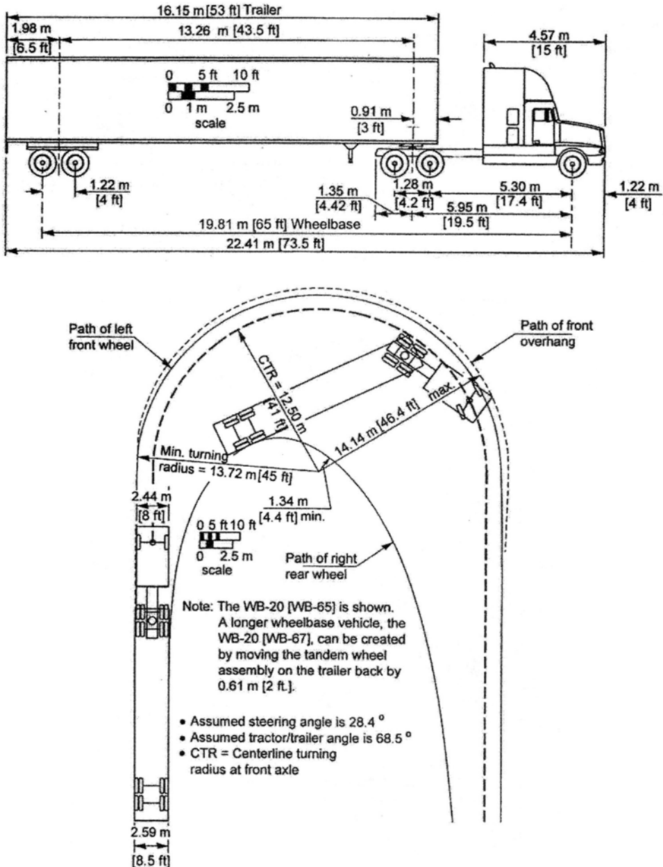
Figure 3.3 Minimum Turning Path for Interstate Semitrailer (WB-20 [WB-65 and WB-67]) Design Value
