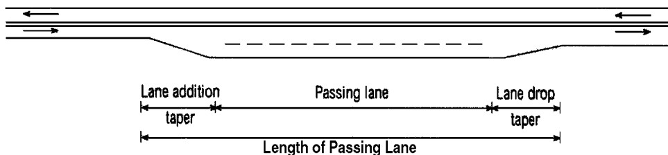
Figure 9.4 Plan View of a Typical Passing Lane
