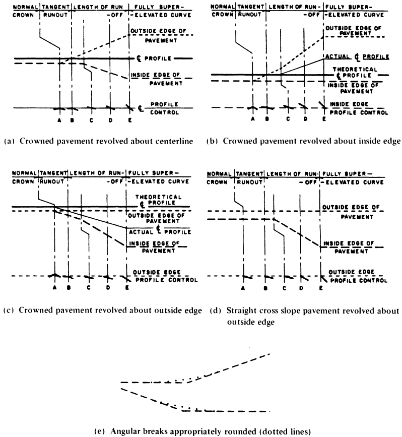
Figure 15.25 Diagrammatic Profiles Showing Methods of Attaining Superelevation for a Curve to the Right
