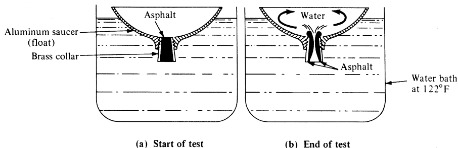
Figure 18.5 Float Test
