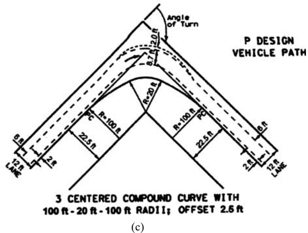
Figure 7.9 Minimum Designs for Passenger Vehicles
