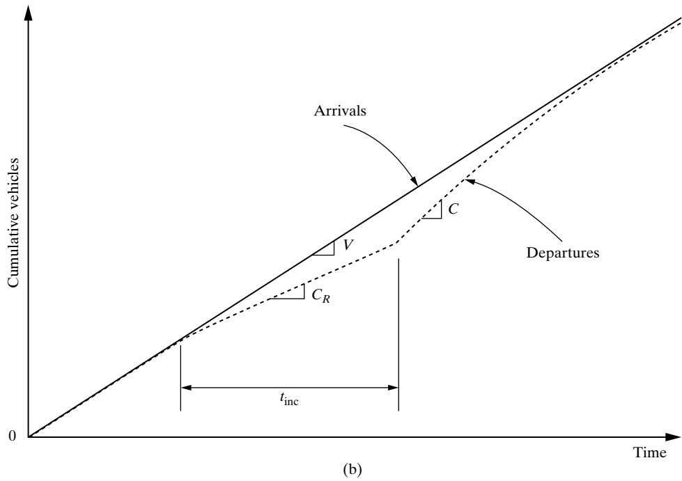
Figure 6.15 Queuing Diagram for Incident Situation
