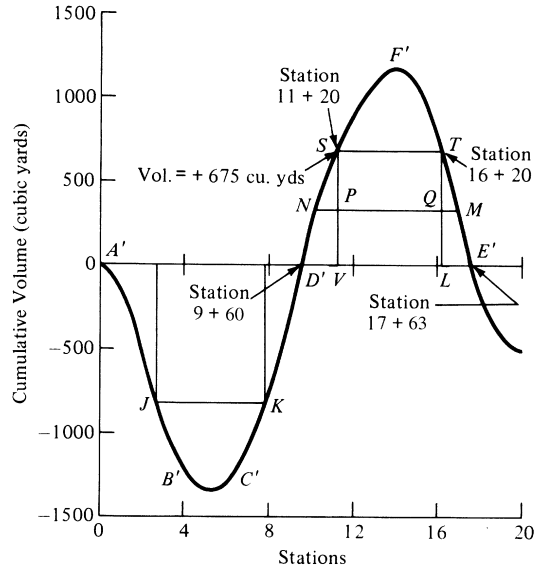
Figure 14.17 Mass Diagram for Computation Shown in Table 14.1
