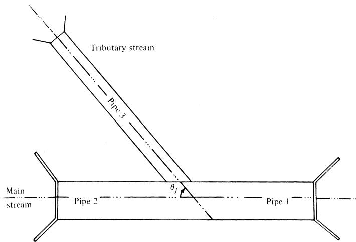
Figure 16.19 Culvert Junction
