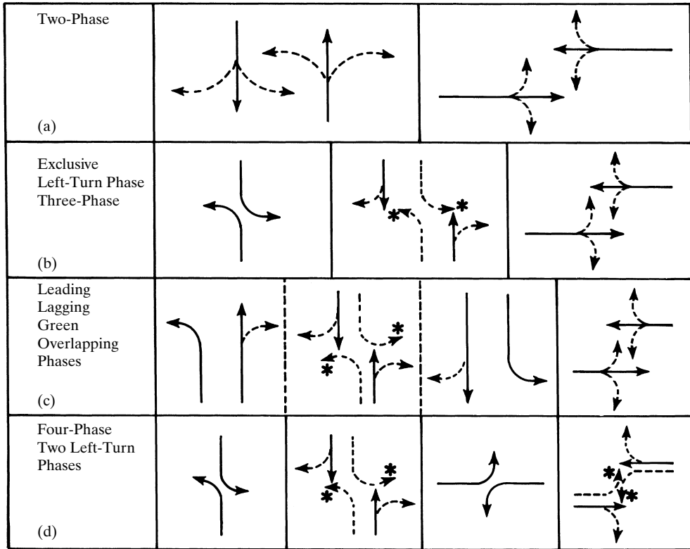
Figure 8.14 Phase Plans for Pretimed and Actuated Signals
