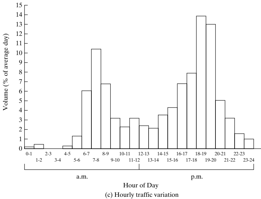
Figure 4.15 Traffic Volumes on an Urban Highway
