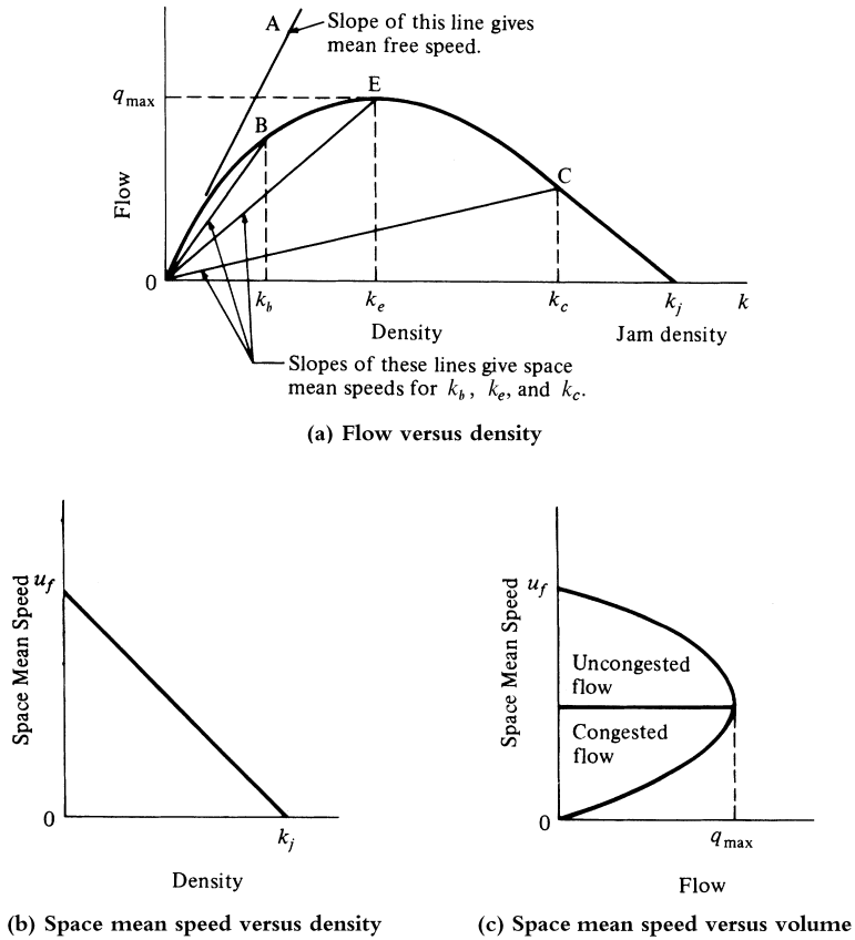
Figure 6.4 Fundamental Diagrams of Traffic Flow
