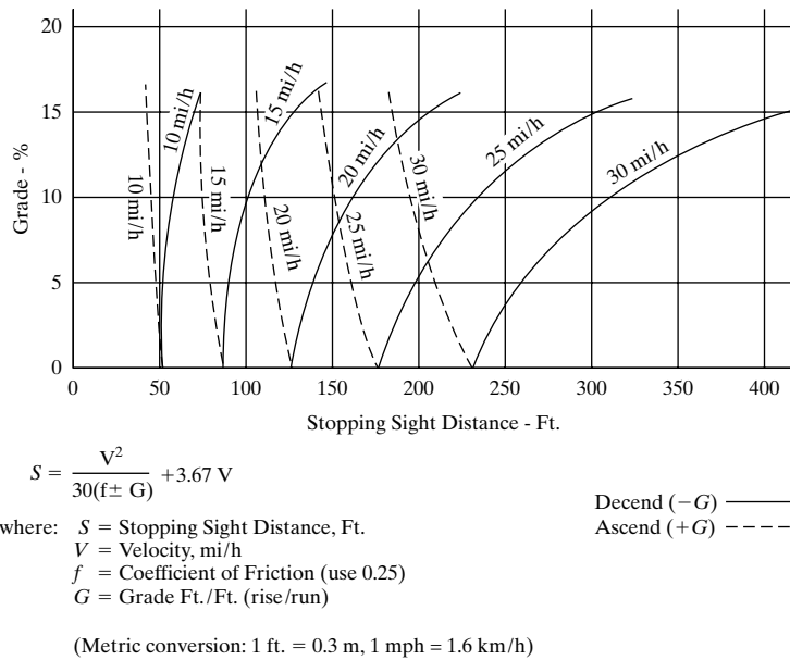
Figure 15.31 Stopping Sight Distance for Bicycles
