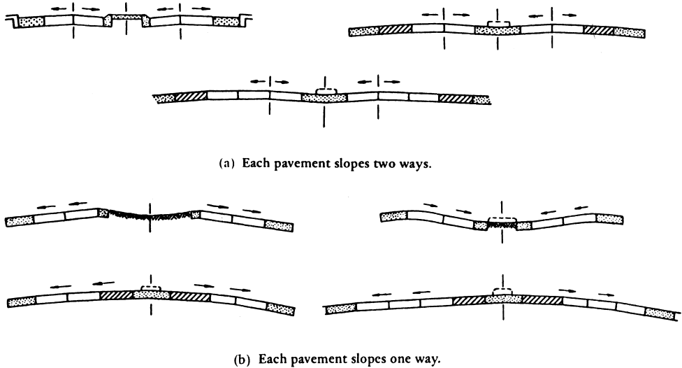
Figure 15.9 Basic Cross Slope Arrangements for Divided Highways
