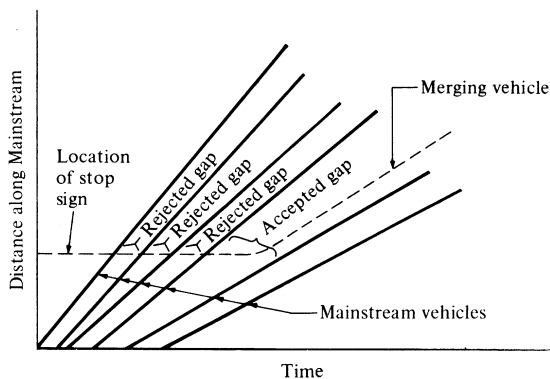
Figure 6.13 Time-Space Diagrams for Vehicles in the Vicinity of a Stop Sign
