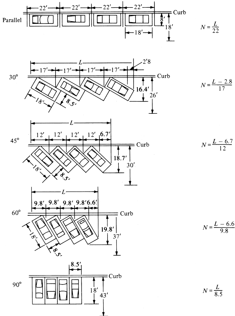
Figure 15.33 Street Space Used for Various Parking Configurations
