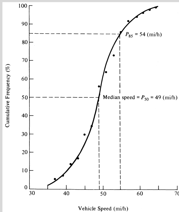
Figure 4.6 Cumulative Distribution
