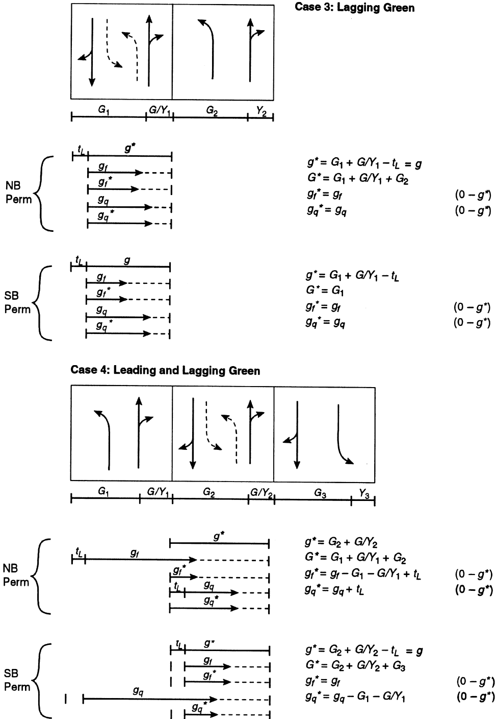
Figure 10.6 Green Time Adjustments for Protected-Plus-Permitted Phasing ( continued )
