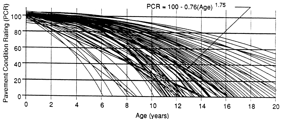
Figure 21.14 Pavement Condition versus Pavement Age
