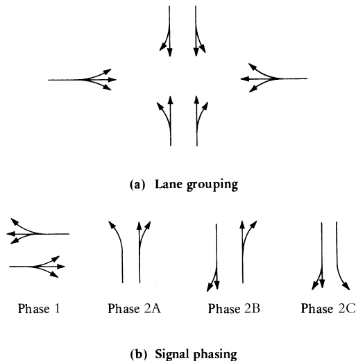
Figure 10.11 Illustrative Example for Determining Critical Lane Group
