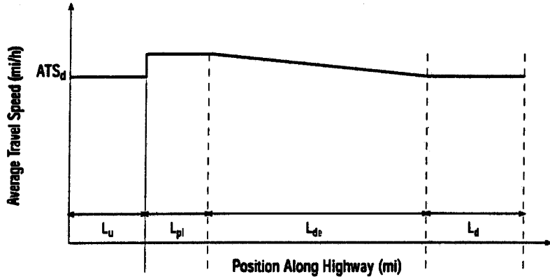
Figure 9.6 Effect of a Passing Lane on Average Travel Speed as Represented in the Operational Analysis Methodology
