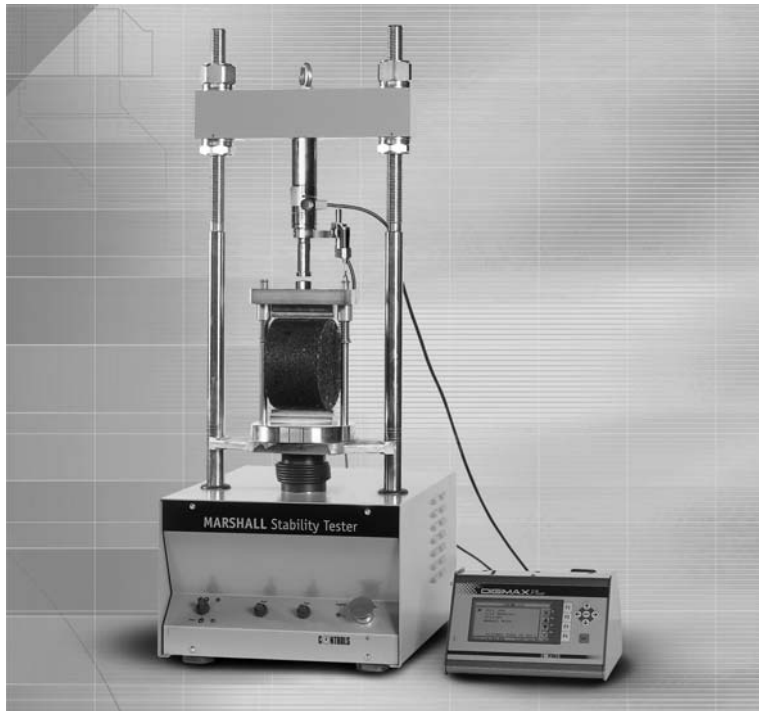
Figure 18.12 Marshall Stability Equipment
