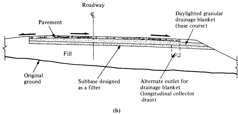
Figure 16.33 Applications of Horizontal Drainage Blankets
