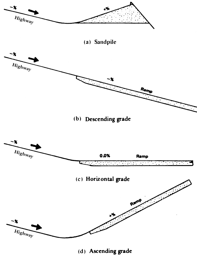
Figure 15.27 Basic Types of Emergency Escape Ramps
